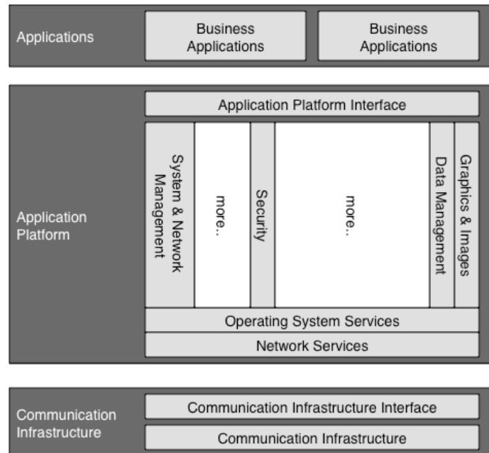
Figure 15: Simplified view upon the TOGAF TRM Overview. For the analogous figure in TOGAF 9.1 see Figure 43-2.
